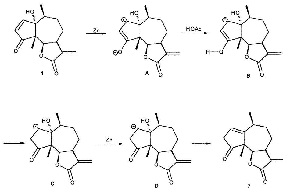
Scheme 2: Formation of 7 from 1 by treatment with Zn/HOAc
