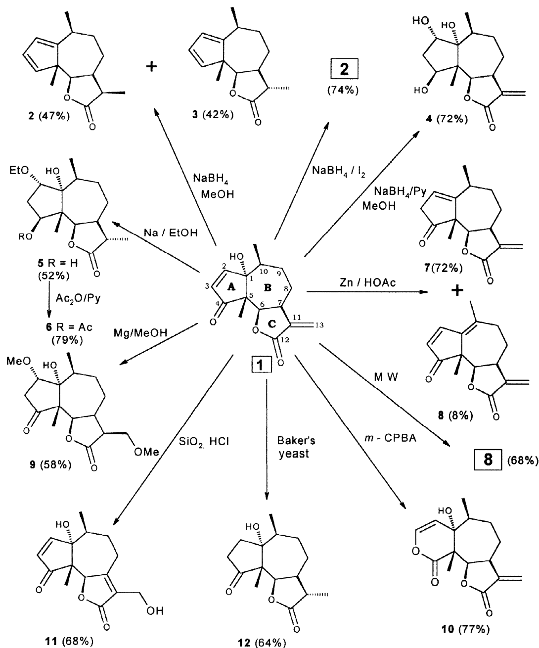
Scheme 1: Reactions of Parthenin 1
